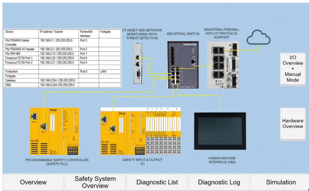
Figure 7 System architecture with security capabilities
